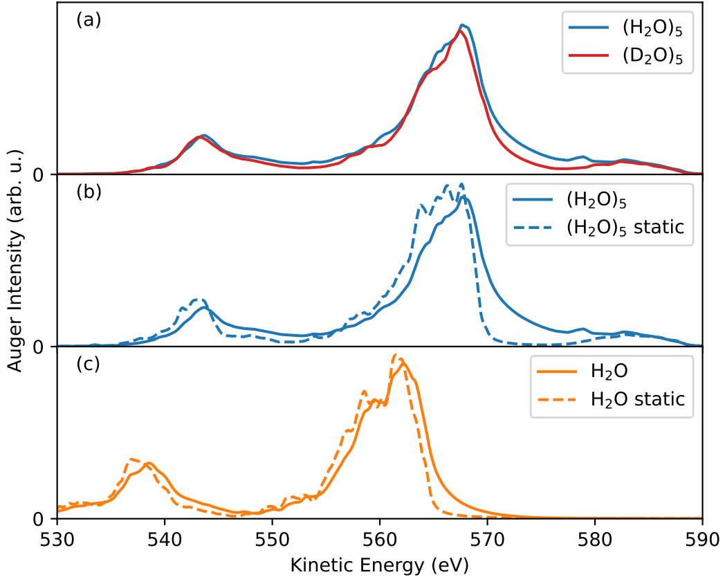
FIG. 5. Calculated Auger electron spectrum. (a) Comparison for the deuterated [(D 2 O) 5 ] and non-deuterated [(H 2 O) 5 ] water pentamer in a tetrahedral arrangement. (b) Auger spectrum for the water pentamer [(H 2 O) 5 ]. (c) Auger spectrum for isolated water (H 2 O). The dashed lines in panels (b) and (c) show instantaneous spectra at t = 0 , i.e., without taking into account the effect of core-hole-lifetime nuclear dynamics.
