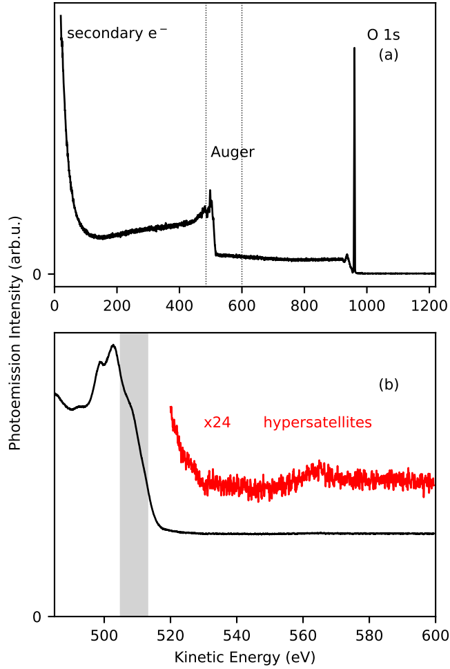
FIG. 2. (a) Full experimental photoemission spectrum of liquid water, excited with photons of 1500 eV. The kinetic-energy interval shown in the lower panel is marked by vertical dotted lines. (b) Photoemission spectrum of liquid water showing the kinetic-energy region of Auger decay marked in panel (a), here recorded at h\nu = 1400 eV. Normal KVV Auger decay can be seen between 480 and 515 eV. The gray-shaded region from 505 to 513 eV kinetic energy is associated with proton-transferred states, for which the nuclear dynamics in the K -shell-ionized state plays a particular role. 4,10 Auger decay of the DCH states, 'hypersatellites', is much weaker due to the low cross section of DCH production by a single photon, and is shifted to substantially higher kinetic energies. The upper trace in panel (b) shows a portion of the spectrum multiplied by 24 and vertically offset to improve its visibility.
