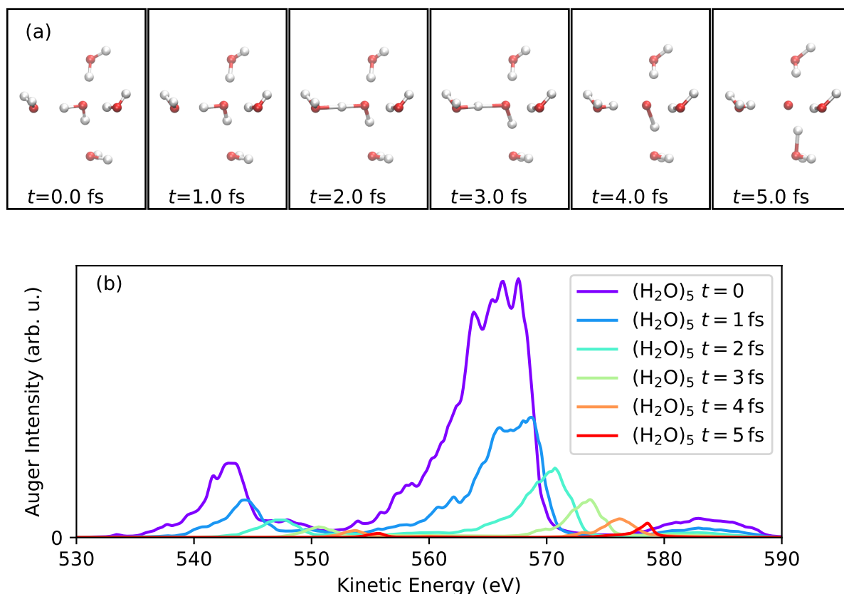
FIG. 6. (a) Snapshots of the molecule geometry for a typical (\text{H}_2\text{O})_5 trajectory. (b) Calculated instantaneous Auger spectra at selected times after core ionization.
