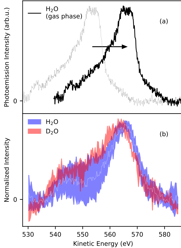
FIG. 4. Auger hypersatellite spectra of O 1s DCHs in gaseous (a) and liquid water (b). The data for gaseous water (dotted line) were shifted by 12.5 eV (horizontal arrow) to allow for an easier comparison and were published in Ref. 20. For the liquid, spectra were measured for normal and deuterated water. The colored error band depicts the standard deviation of several, independently acquired data sets. For normal water, the average is indicated by a thin dotted line.
