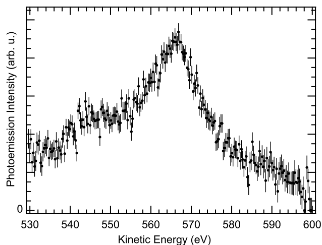
FIG. 3. Close-up on the photoemission intensity from liquid water on the high-kinetic-energy side of the normal Auger spectrum, recorded with a photon energy of 1400 eV. The feature between 560-570 eV of kinetic energy is identified with the first step Auger decay of a DCH in liquid water. A linear background has been subtracted. See text for details.
