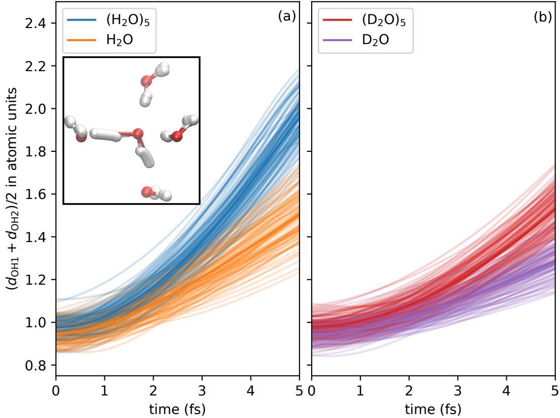
FIG. 7. Symmetrized oxygen-hydrogen distance as function of time after double core ionization. (a) Comparison of water pentamer in a tetrahedral arrangement [(\text{H}_2\text{O})_5] and isolated water ( \text{H}_2\text{O} ). The inset illustrates an example trajectory for the pentamer [see Fig. 6(a) for individual snapshots]. (b) Comparison of deuterated [(\text{D}_2\text{O})_5] water pentamer and isolated deuterated water.
